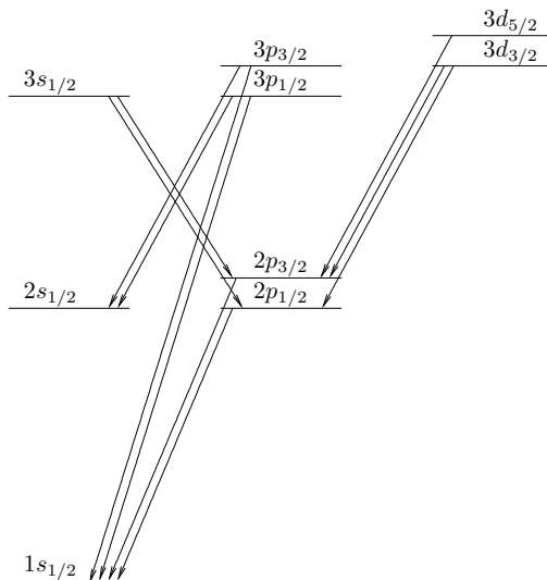
Fig. 2. Energy level diagram for hydrogen or hydrogen-like atoms, including fine structure, with allowed electric dipole transitions indicated (Grotrian diagram). Not shown are transitions only involving small energy differences, such as 3p_{3/2} \rightarrow 3s_{1/2} . Diagram is schematic and not to scale; in particular, the fine structure splittings are of order (Z\alpha)^2 times the separation between the levels of different n .
