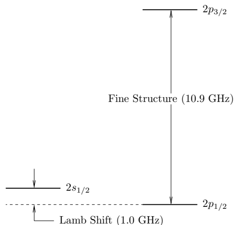
Fig. 3. An expanded view of the n = 2 levels in hydrogen, including the Lamb shift. The splitting due to the Lamb shift is notable because it introduces an \ell -dependence into the energies. Its magnitude is about 10 times smaller than the fine structure splitting (on the n = 2 levels).
