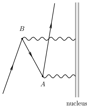
Fig. 1. Feynman diagram for the creation of an electron-positron pair in the orbital motion of an electron in the hydrogen atom. The diagram is a space-time diagram with time increasing vertically, with the world-lines of the nucleus and electrons and a positron shown. Starting at the bottom, the electron in orbit around the nucleus enters at the left. Electron world-lines are indicated with an arrow pointing in the direction of increasing time. Later, at space-time point A , a photon from the nucleus creates a positron electron pair, so that for a time there exist two electrons and one positron in the system. The positron world line is indicated with an arrow pointing backwards in time. At a later time, at space-time point B , the incoming electron annihilates with the positron, producing a photon that is absorbed by the nucleus. After this, a single electron continues in its orbit, but, in a sense, it is not the same electron that entered at the bottom. The effect of diagrams like this is to smear the position of the atomic electron around in space over a distance comparable to the Compton wavelength.
